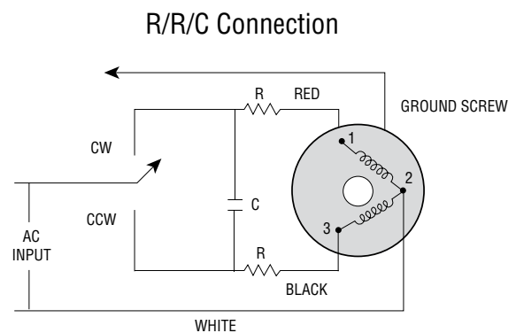
Two-Phase Operation
