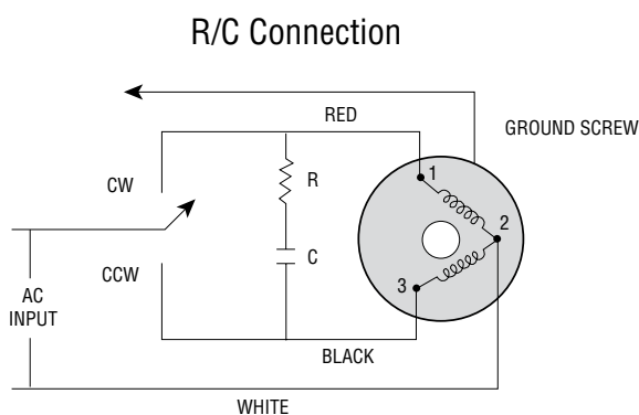
Single-Phase Operation
