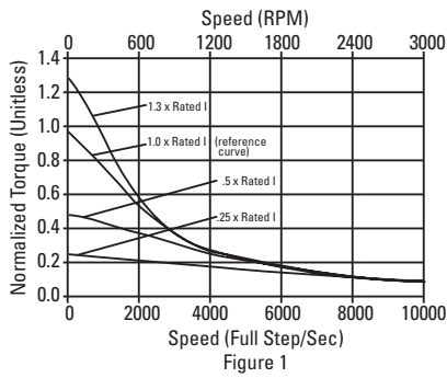
Figure 1 shows the performance of a motor with different drive current settings and the same supply voltage. Note that low speed running torque varies considerably with changes in drive current setting, but high speed performance is not appreciably affected.
