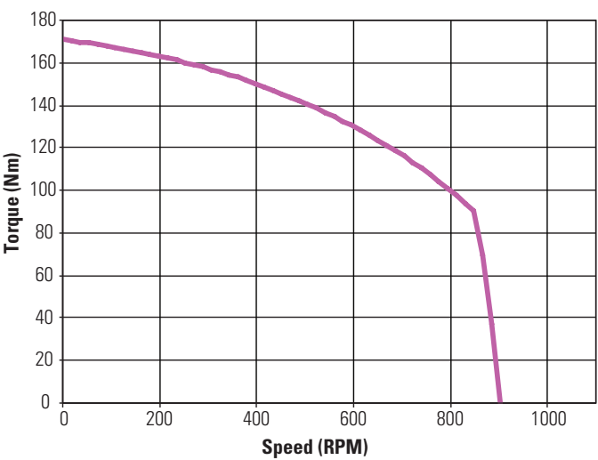
KBM(S)-118X00 ContinuousTorque
