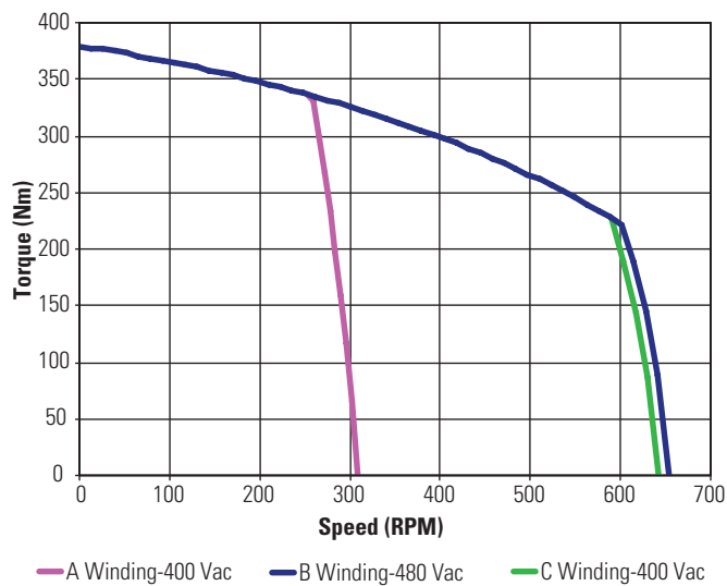
KBM(S)-88X02 ContinuousTorque
