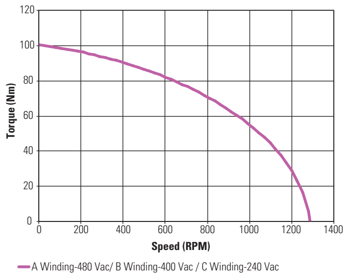
KBM(S)-88X00 ContinuousTorque
