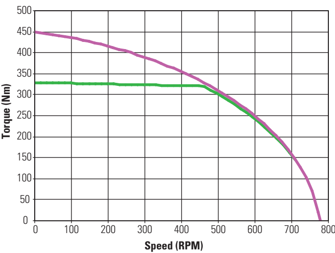
KBM(S)-118X02 ContinuousTorque
