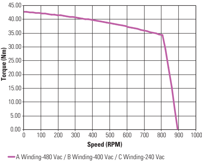
KBM(S)-79X01 ContinuousTorque
