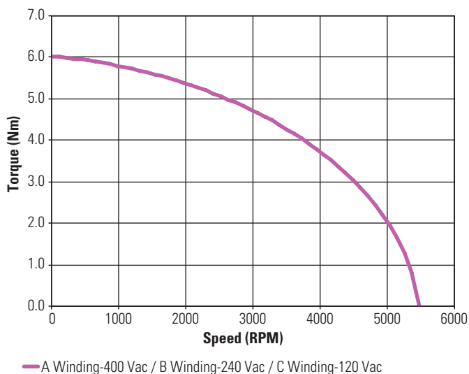
KBM(S)-43X01 ContinuousTorque
