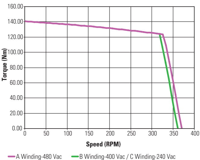
KBM(S)-79X03 ContinuousTorque
