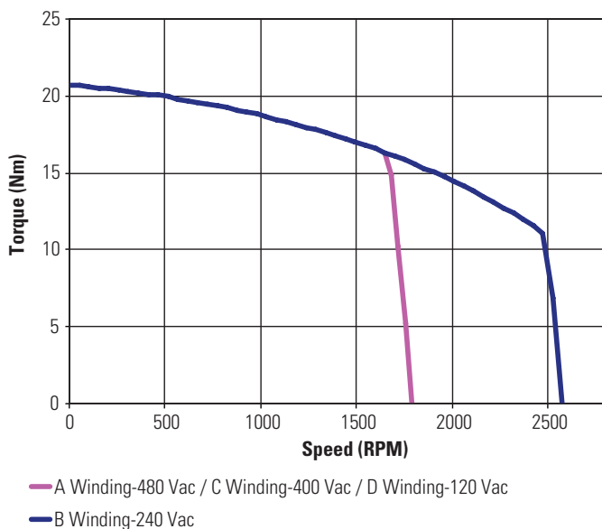
KBM(S)-43X03 ContinuousTorque
