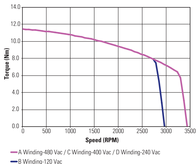
KBM(S)-43X02 ContinuousTorque
