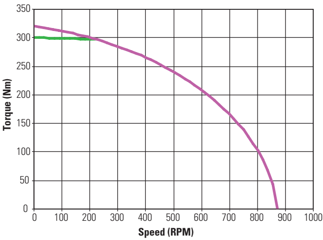
KBM(S)-118X01 ContinuousTorque
