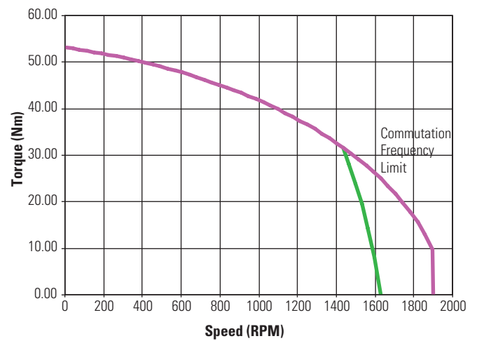
KBM(S)-60X01 ContinuousTorque
