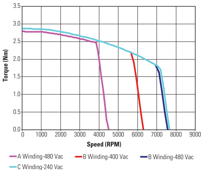
KBM(S)-14X03 ContinuousTorque
