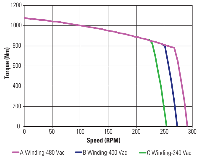
KBM(S)-163X02 ContinuousTorque
