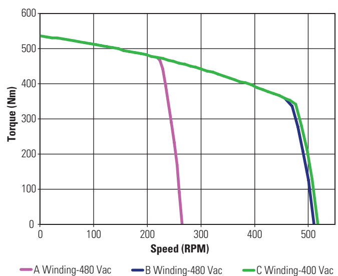
KBM(S)-88X03 ContinuousTorque
