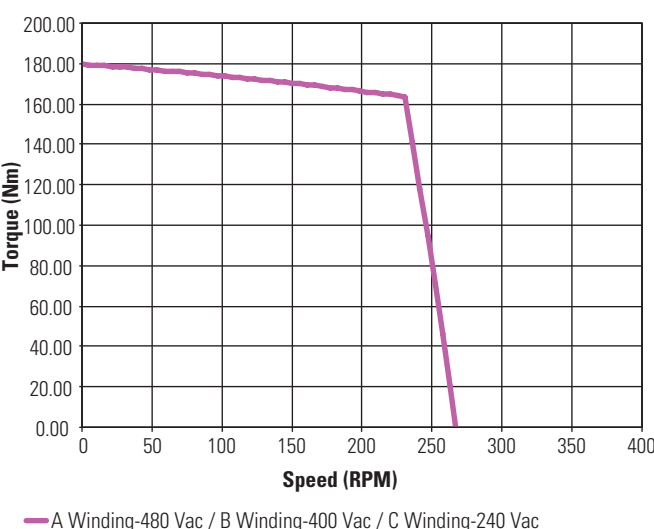
KBM(S)-79X04 ContinuousTorque
