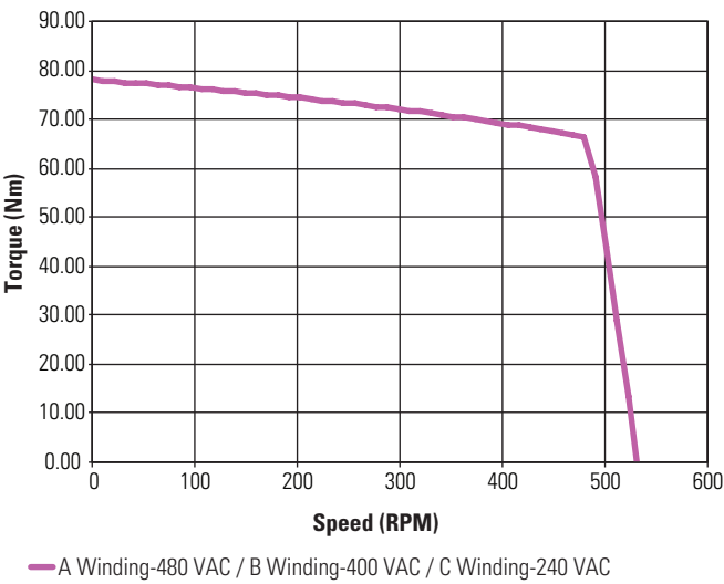
KBM(S)-79X02 ContinuousTorque
