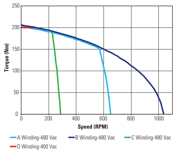
KBM(S)-88X01 ContinuousTorque
