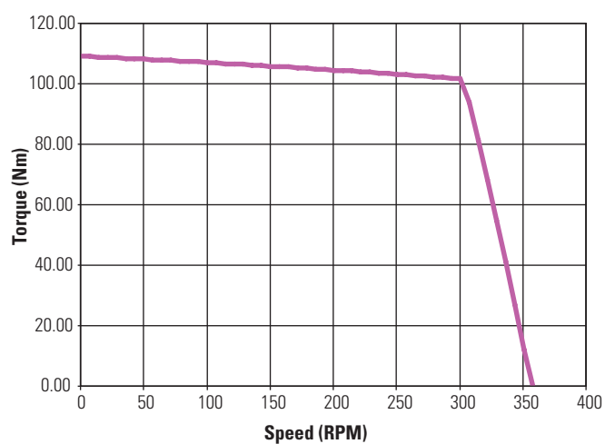
KBM(S)-57X05 Continuous Torque
