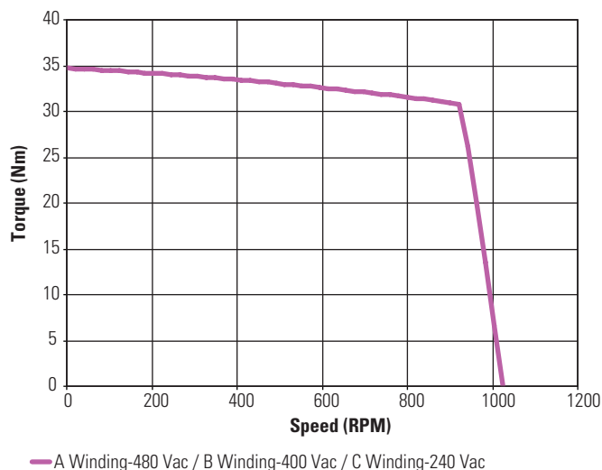
KBM(S)-43X04 ContinuousTorque
