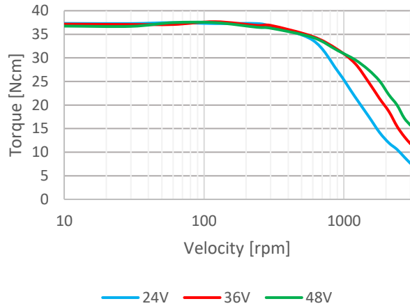
Pull-out torque HL12 2,0A
