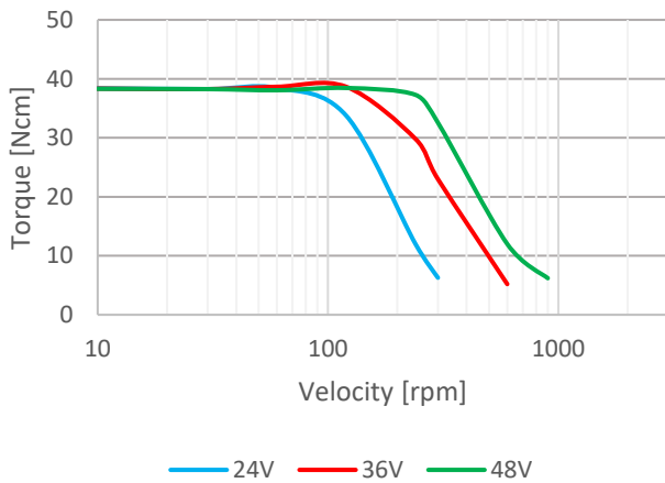
Pull-out torque HL12 0,4A
