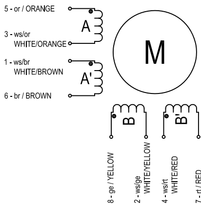
Anschlußplan SL20 - 22 Serie 8 Leiter Conn. Diagram SL20 - 22 Series 8 Leads
