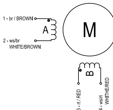
Anschlußplan SL20 - 22 Serie 4 Leiter Conn. Diagram SL20 - 22 Series 4 Leads
