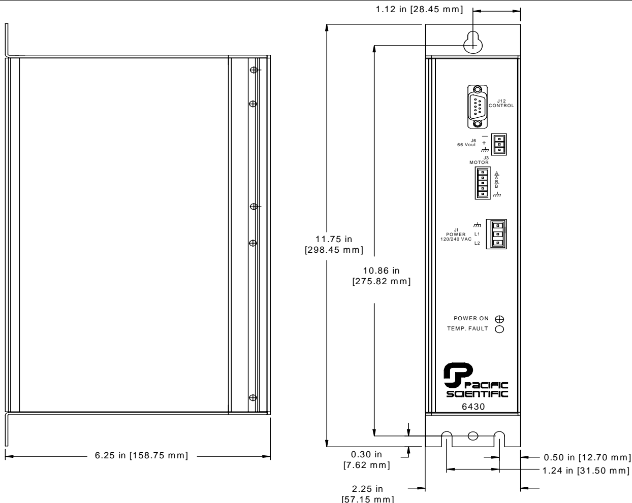
Figure 4 Mounting Dimensions
